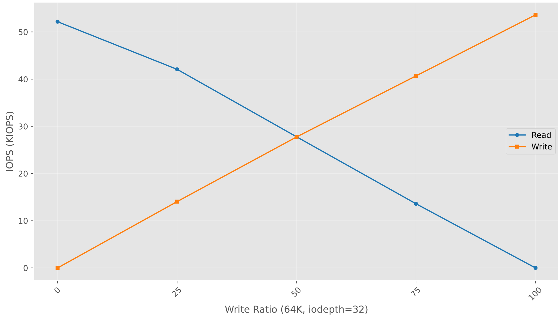
IOPS vs Write Ratio (64K, iodepth=32)
